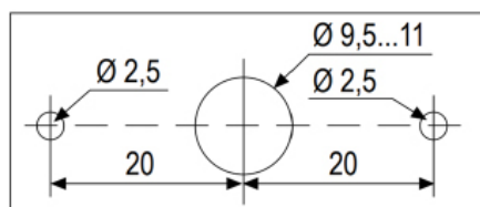
Drill template
